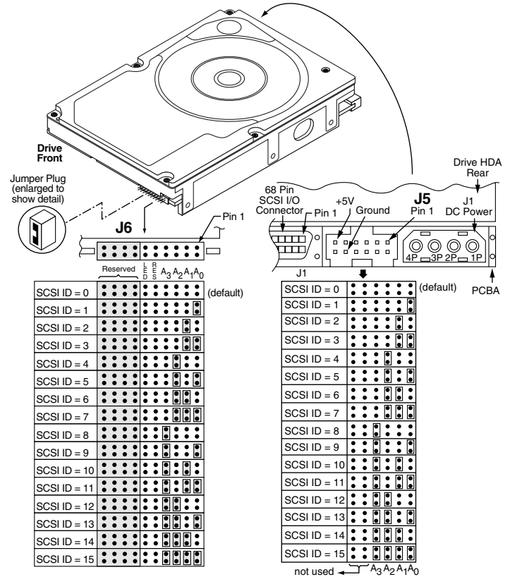
Figure 1. Setting the SCSI ID (the J5 block is on LW models only)
